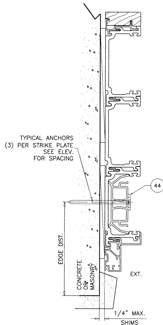
ANCHORS THRU STRIKE PLATE
