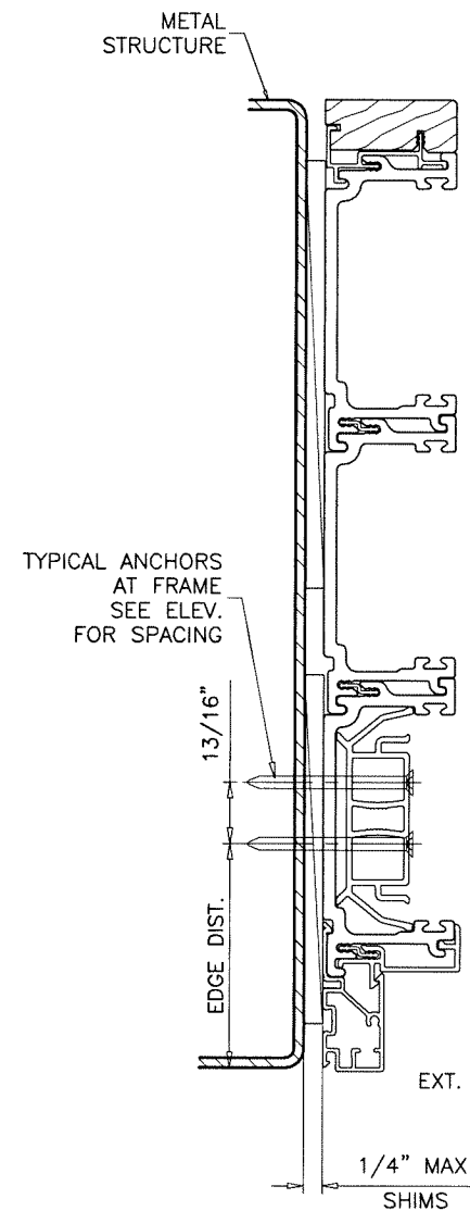
ANCHORS THRU FRAME
